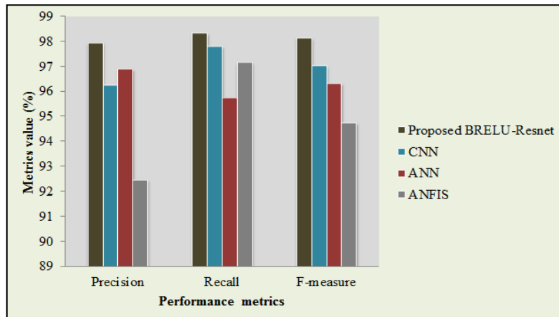
Fig. 5: Comparative analysis of proposed BREL-ResNet based on precision, recall, and F-Measure.
