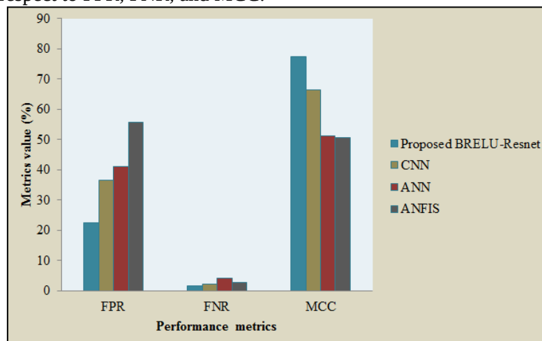
Fig. 6: Comparative analysis of proposed BREL-ResNet in terms of FPR, FNR, and MCC.
